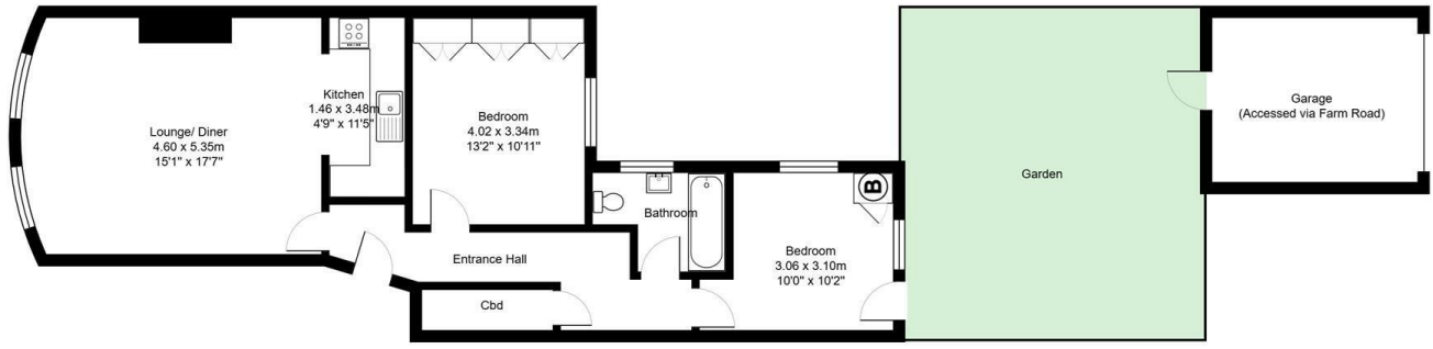
Brunswick Place Total Area: 73.2 m² ... 788 ft² (Excluding Garden & Garage) All measurements are approximate and for display purposes only.
